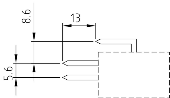
MISURE MICROINTERRUTTORE / microswitch measures
