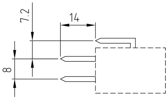
MISURE MICROINTERRUTTORE / microswitch measures
